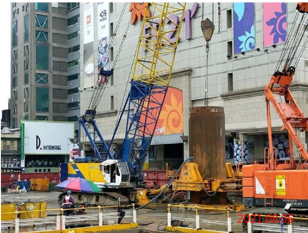
G07 站_全套管基樁及逆打鋼柱樁號抓掘
